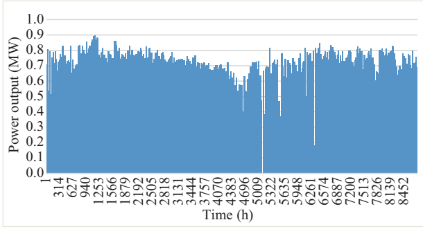
Fig. 4. The unitized power curve of PV plant.
