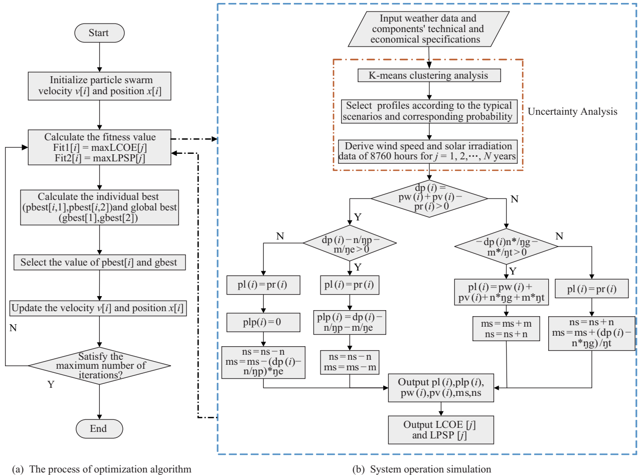
Fig. 3. Flowchart of the proposed probabilistic simulation-based optimization approach.
