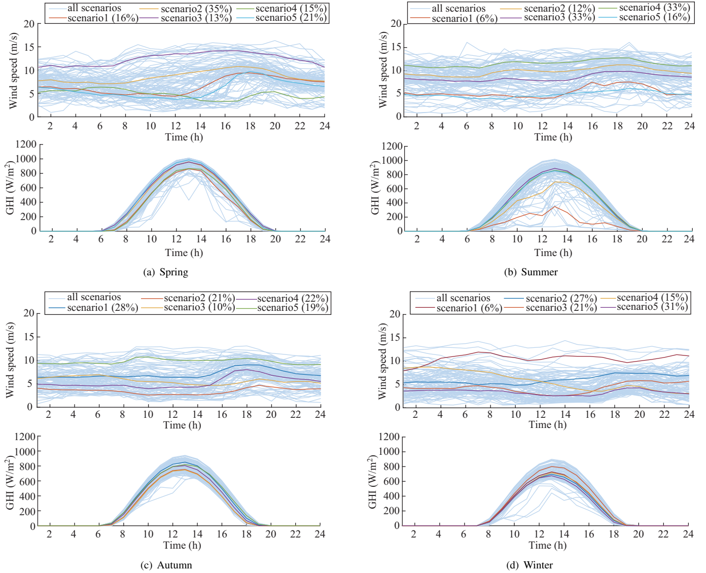
Fig. 2. Typical scenarios of renewable energy and their occurrence probability.
