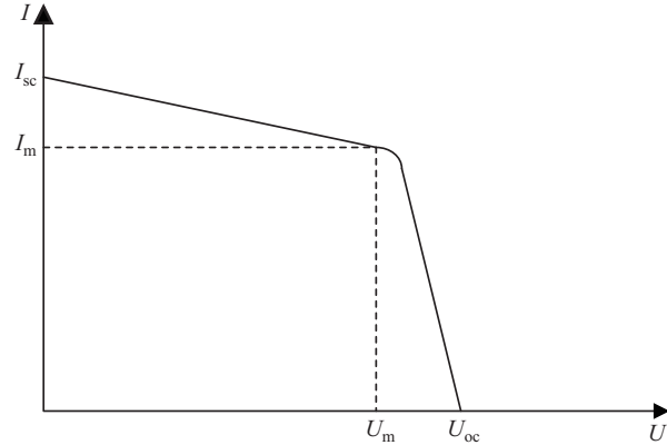
Fig. A2. The I-V curve of SFM260W model [43].
