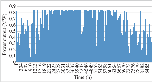
Fig. 5. The unitized power curve of wind farm.
