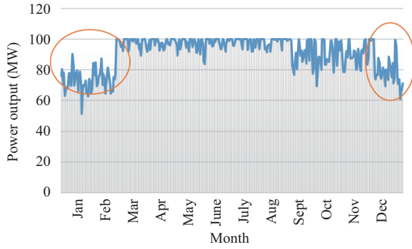
Fig. 8. Power output curve of hybrid power system.
