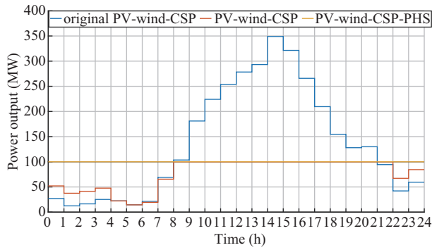
Fig. 10. Power output curve of representative day.
