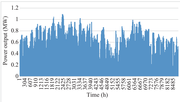
Fig. 6. The unitized power curve of CSP plant (without TES).
