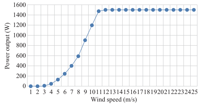
Fig. A1. The wind power curve of UP77-1500 model [42].
