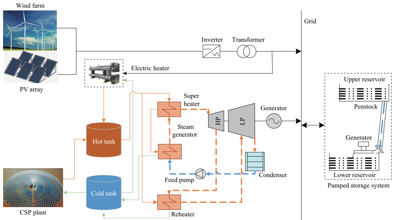
Fig. 1. PV-wind-CSP-PHS hybrid power system.
